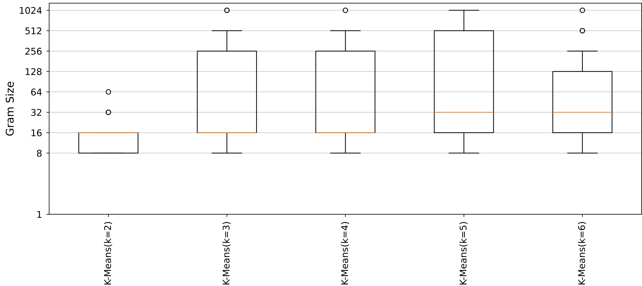
YARA Rules Gram Size Distribution (Cluster21_Size6 dataset)
